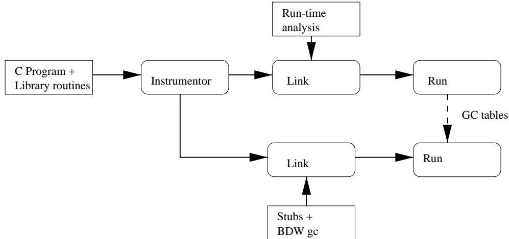
Figure 1: Framework for collecting type-accurate information
