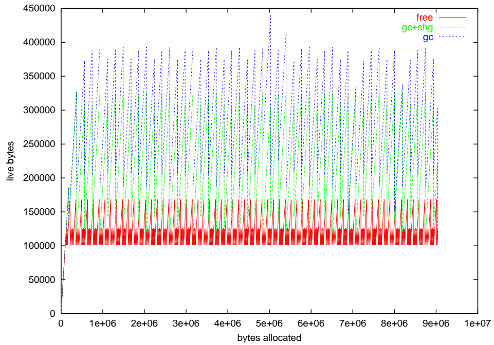
Figure 3: Memory usage of jpeg-50 on a SPARC
