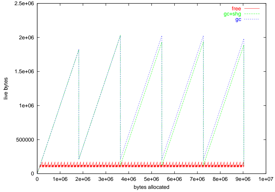
Figure 2: Memory usage of jpeg-5 on a SPARC
